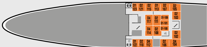
DECK C
